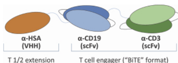
Design of CLN-978, a CD19/CD3-bispecific T Cell Engager with Extended Serum Half-life
